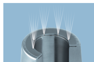
Optimised coolant bores with coolant outlet through slots
