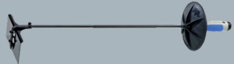
CHIP HOOK WITH SHOVEL SP2740 Length with added modular rod 500 mm.
