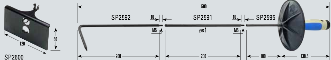
MODULAR DIMENSIONS - metric
